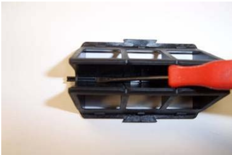
Removal of old reed petal using a screwdriver
